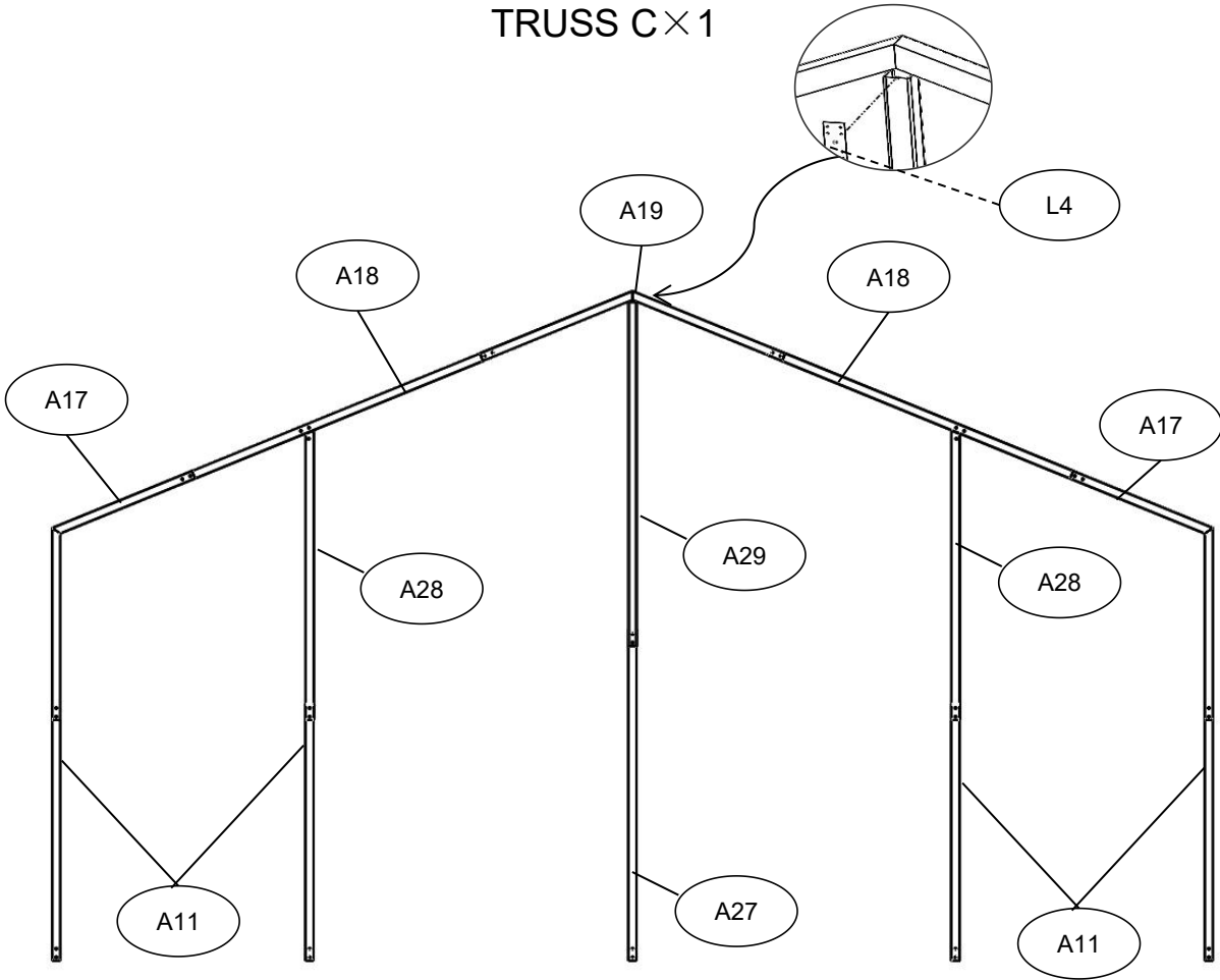
Installation of the rear wall side posts
