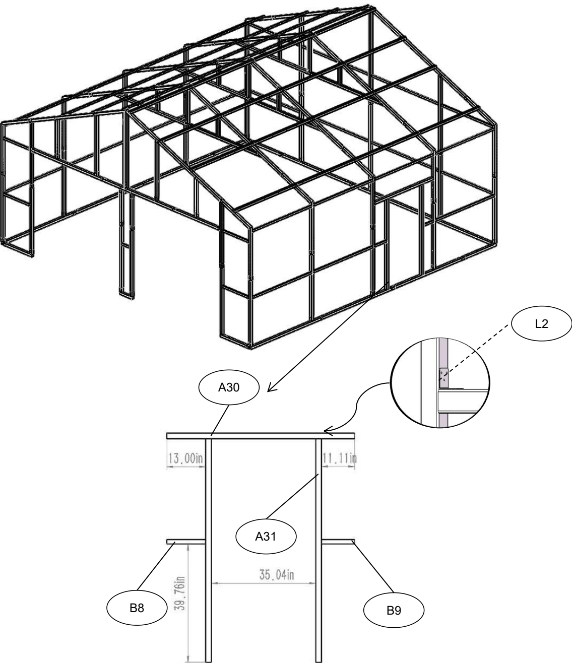
Installation of the side small door frame
