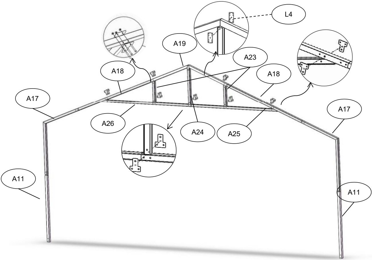
TRUSS B×3
